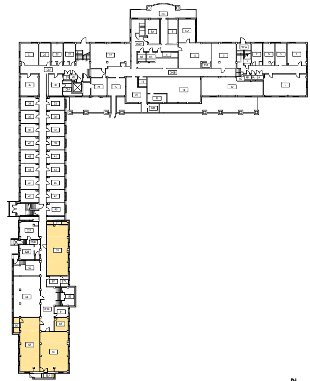
2 CORBIN, N CORBIN & BRANTLY HALLS (BUILDING 913) - BASEMENT LEVEL SCALE: 1/32" = 1'-0" (D SIZE)
