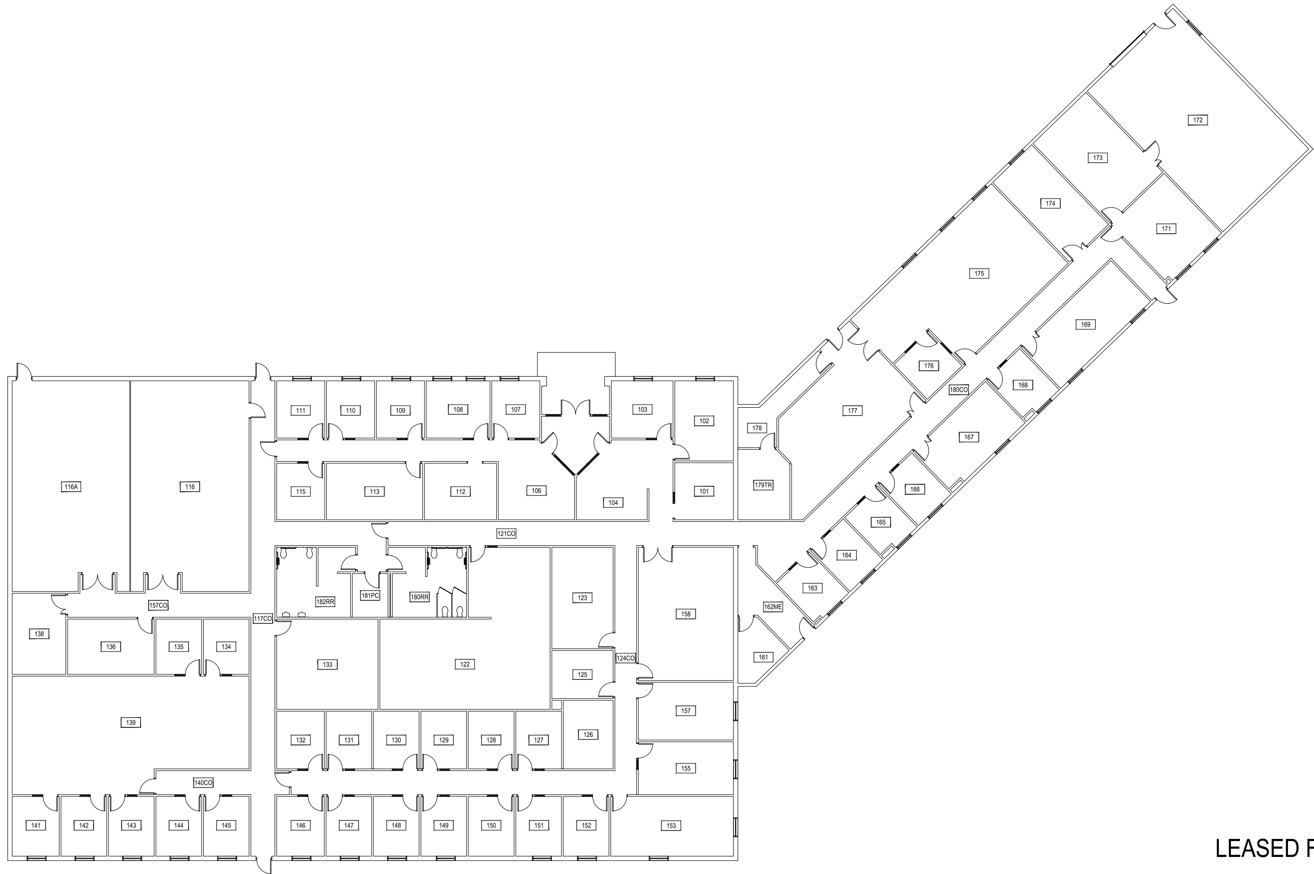
1 CFT BUILDING #2 - FIRST LEVEL SCALE: 1" = 20'
