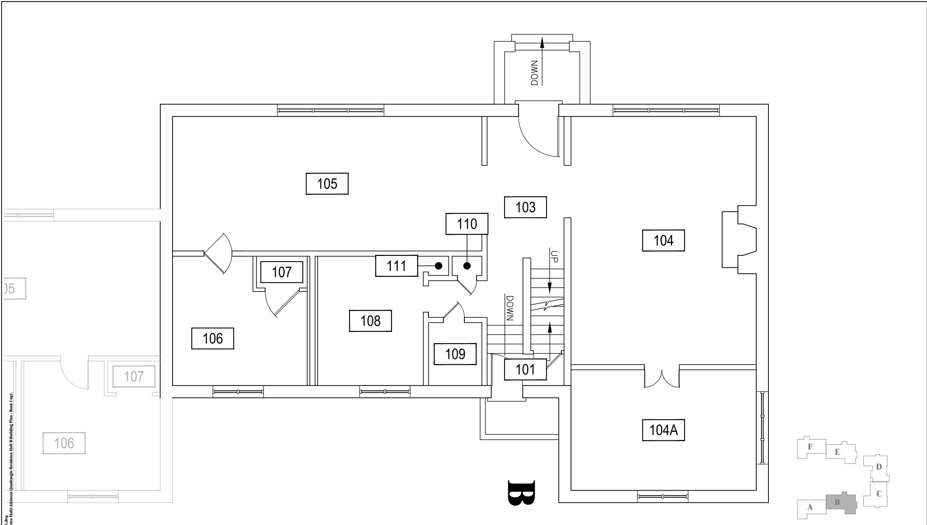
1 ATKINSON QUADRANGLE RESIDENCE HALL B - FIRST LEVEL SCALE: 3/16" = 1'
