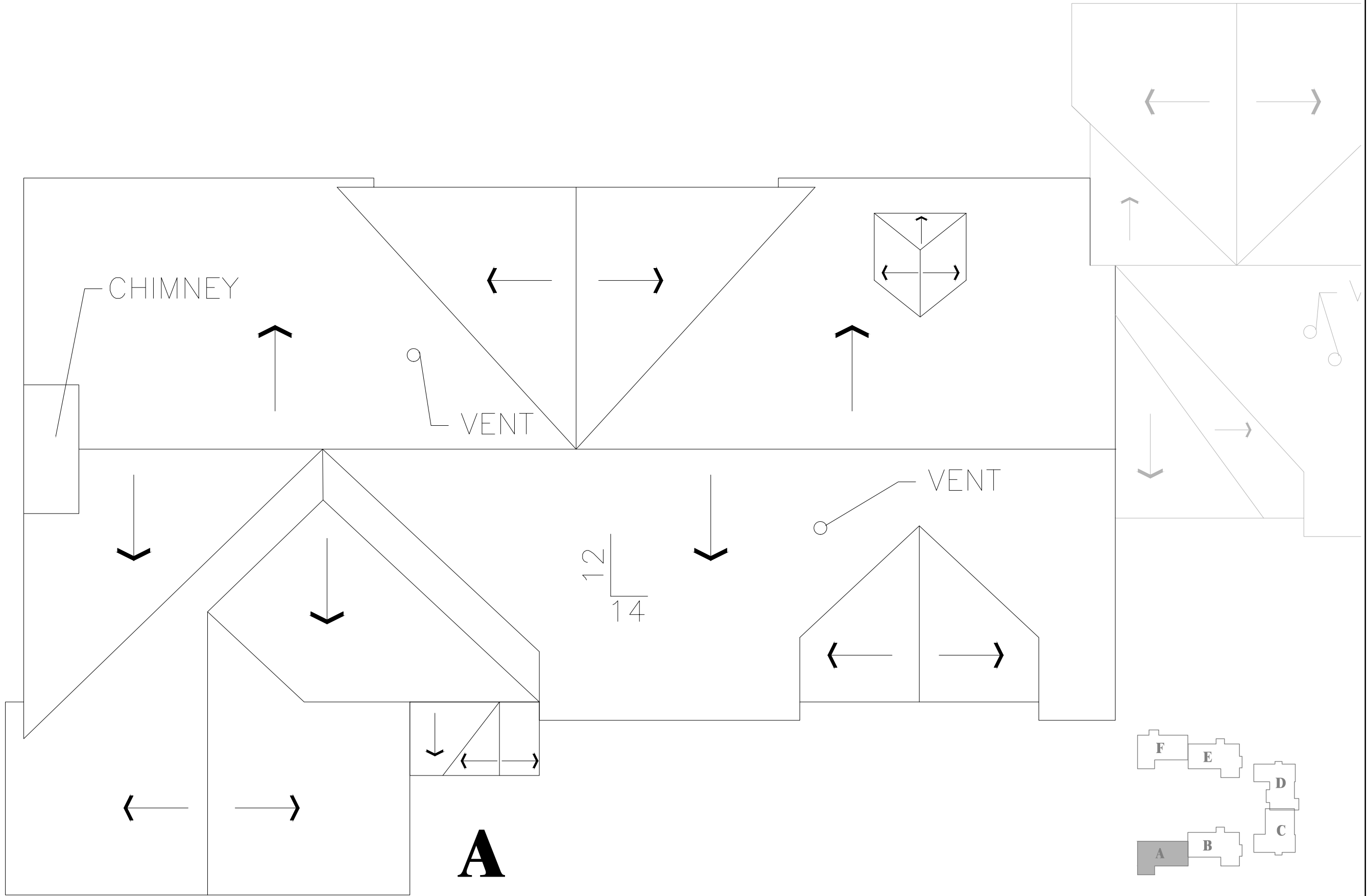
1 ATKINSON QUADRANGLE RESIDENCE HALL A - ROOF LEVEL SCALE: 3/16" = 1'
