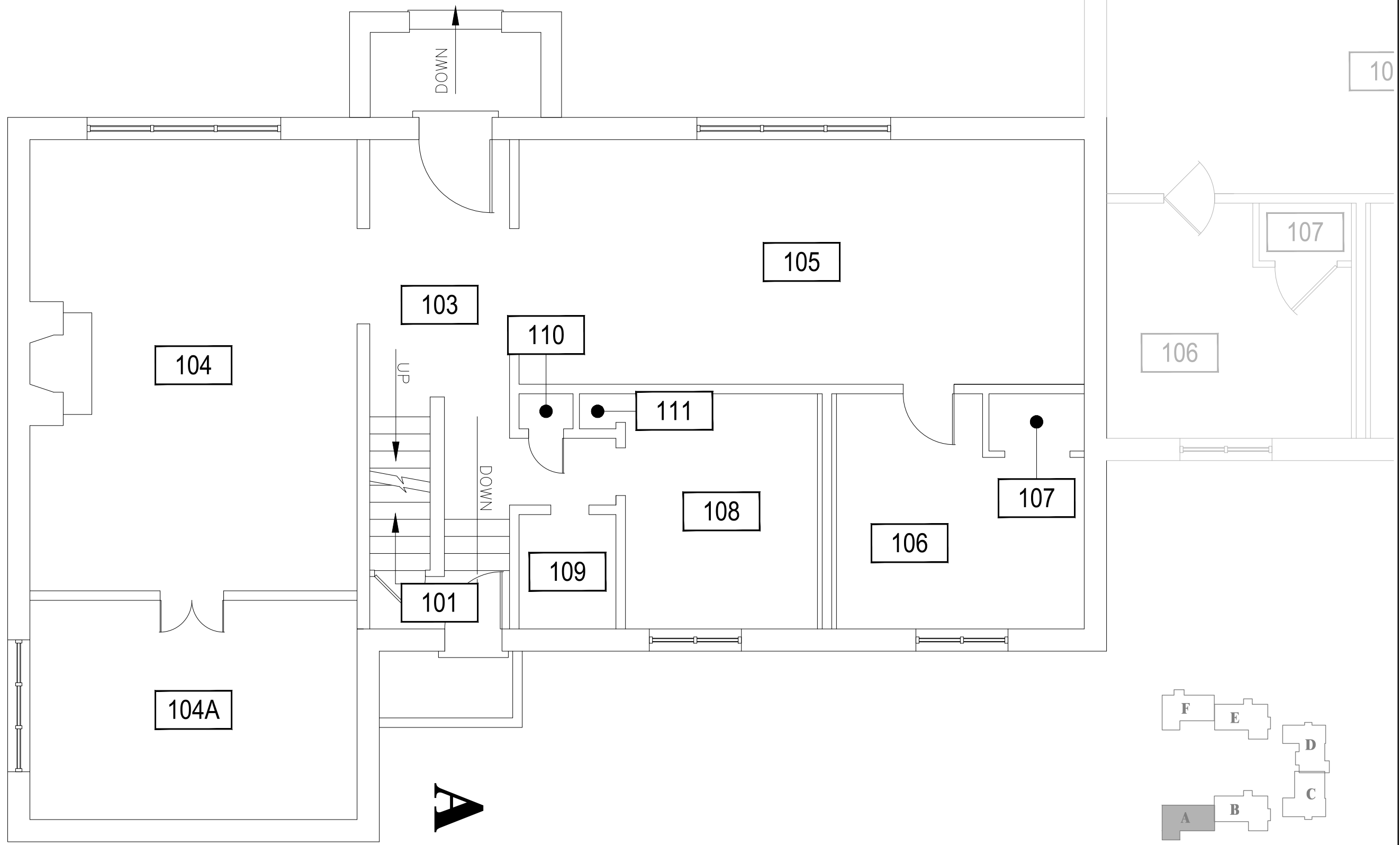
1 ATKINSON QUADRANGLE RESIDENCE HALL A - FIRST LEVEL SCALE: 3/16" = 1'
