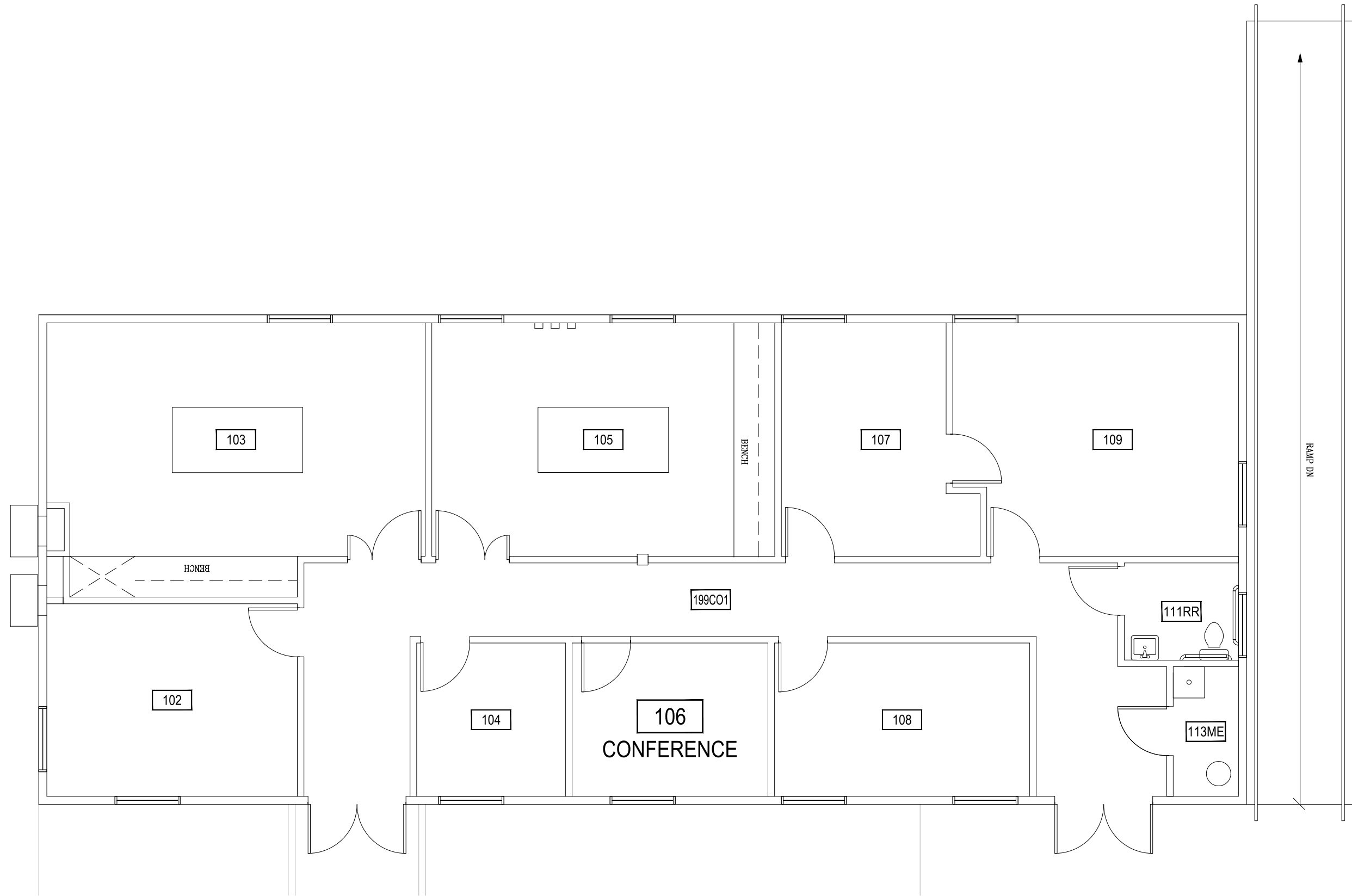
1 FACULTY COURT-11 - FIRST LEVEL SCALE: 5/32" = 1'
