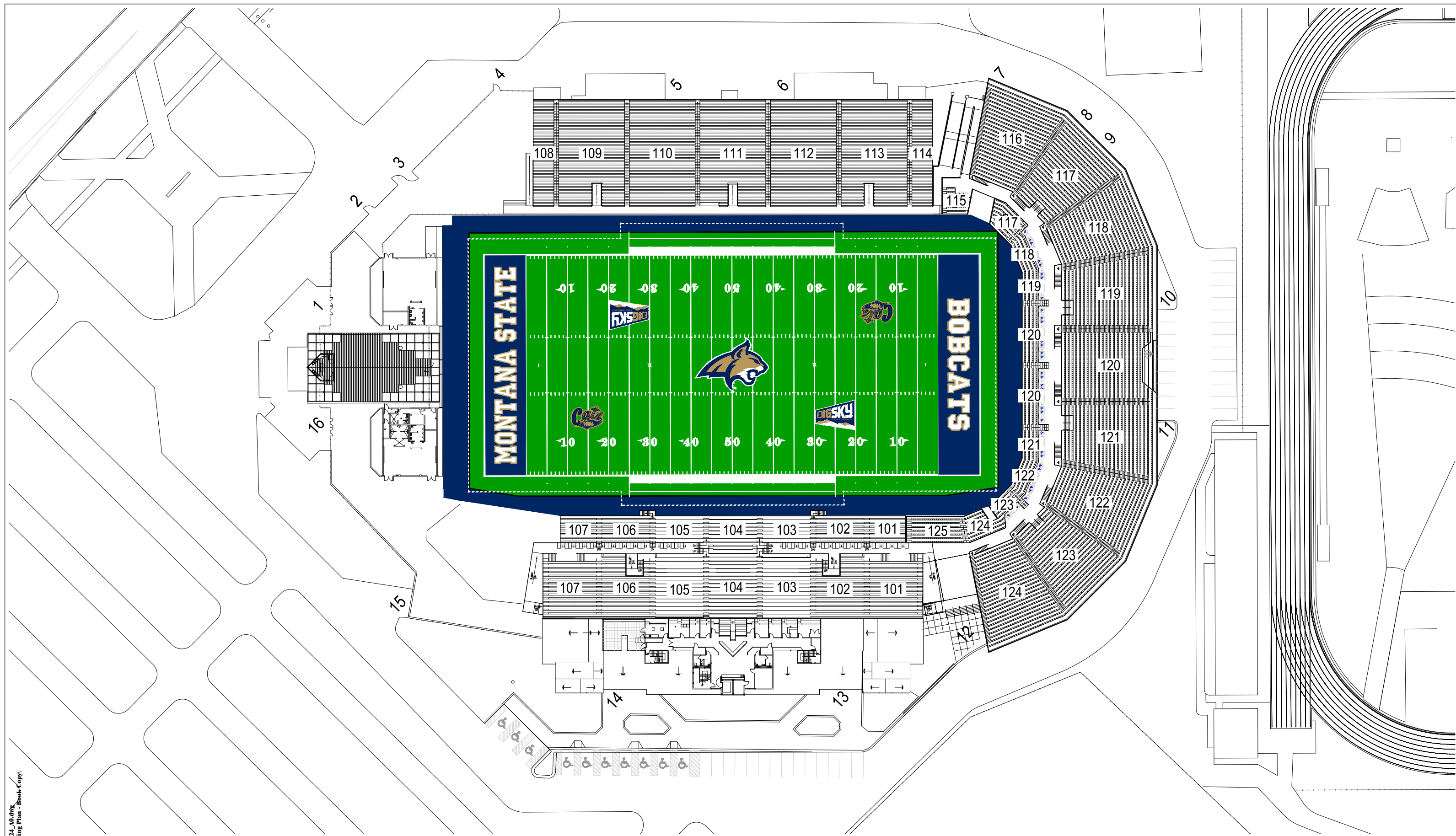
1 BOBCAT STADIUM - PLAN VIEW SCALE: 1/64" = 1'
